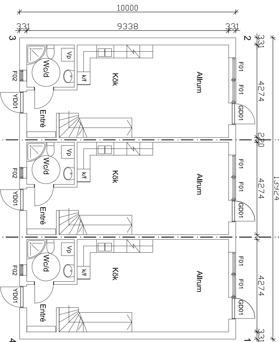
Bottenplan
