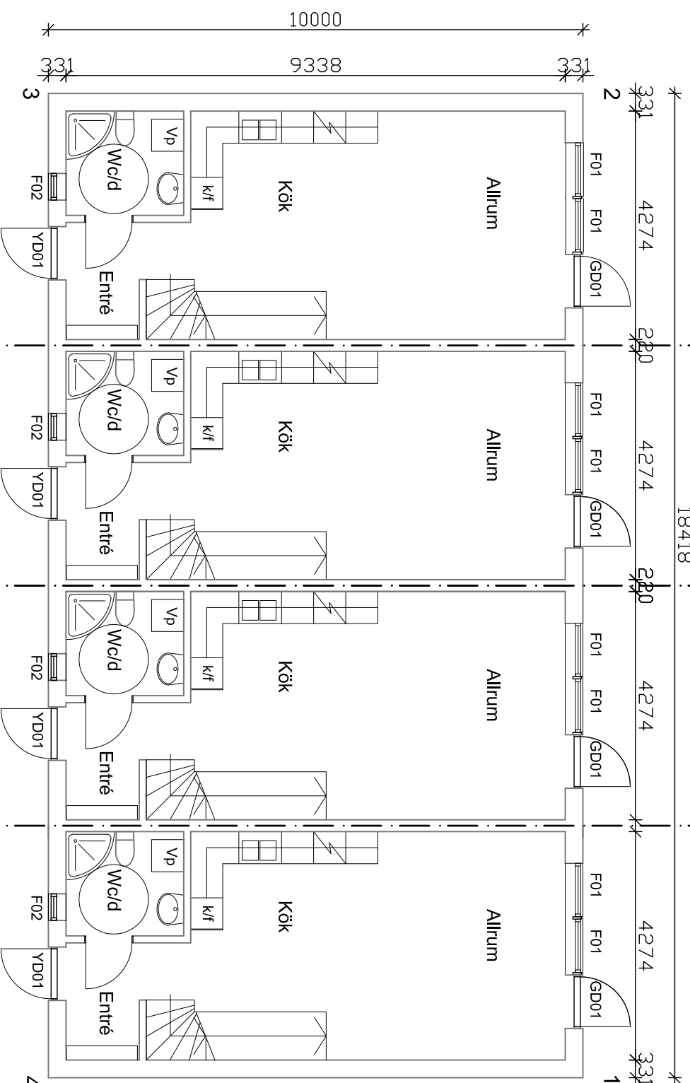
Bottenplan
